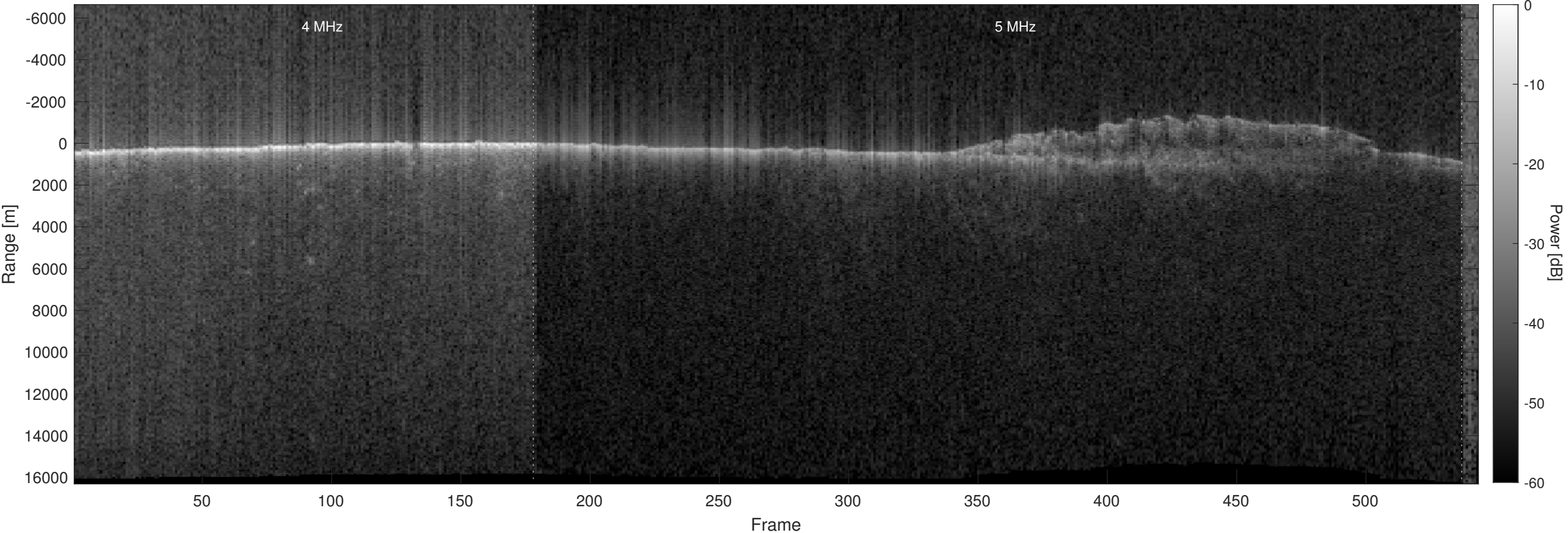
Orbit 22515, Optimized, No Window, Depth-Corrected, Channel 2
