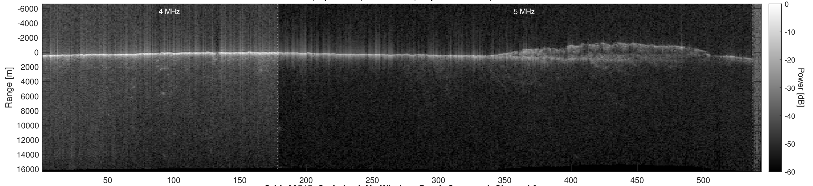
Orbit 22515, Optimized, No Window, Depth-Corrected, Channel 2
