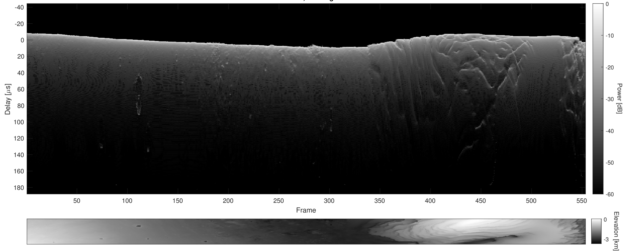
Orbit 22517, Cluttergram
