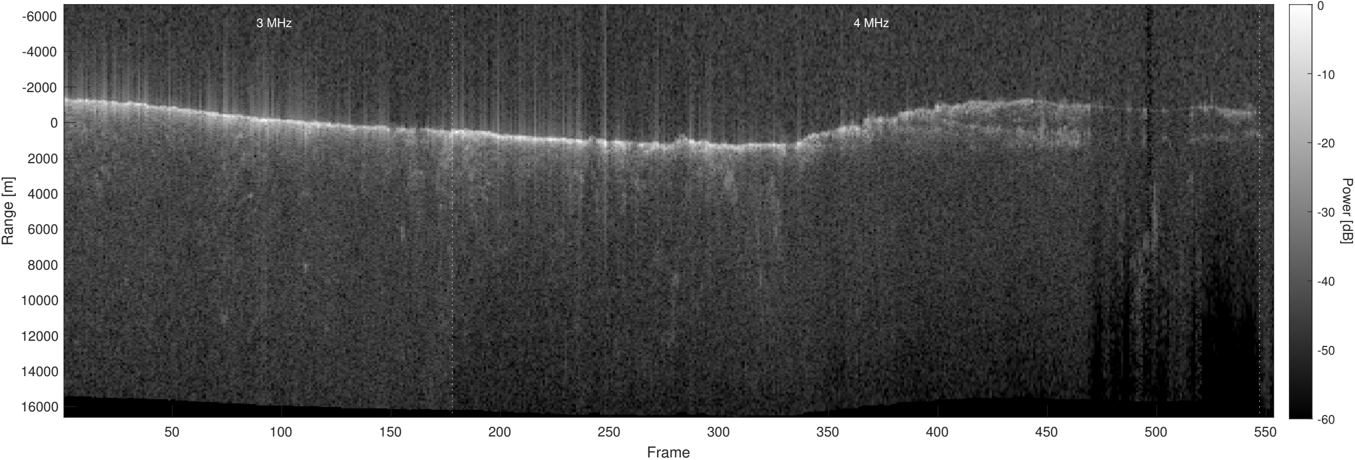
Orbit 22517, Optimized, No Window, Depth-Corrected, Channel 2
