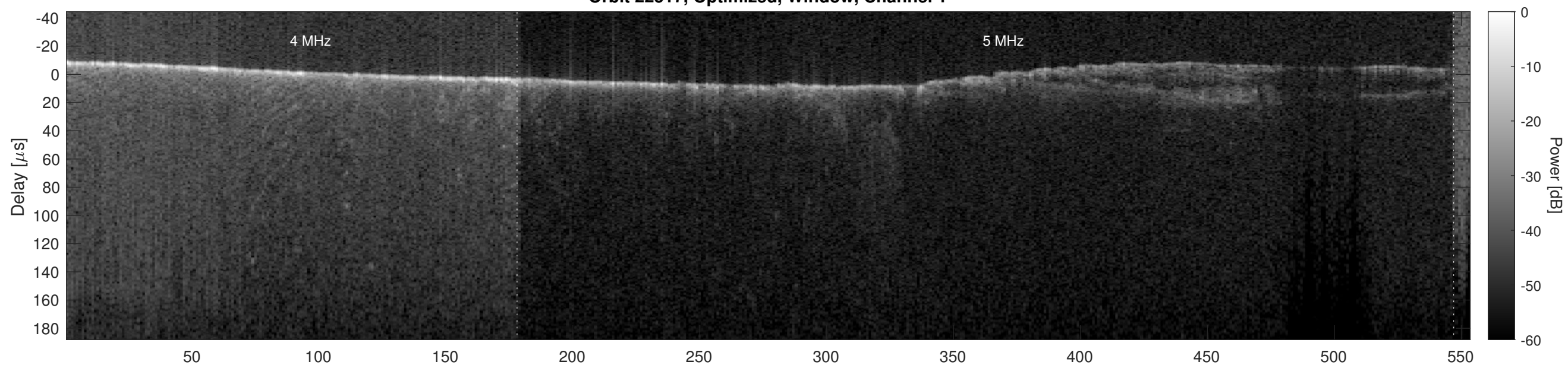
Orbit 22517, Optimized, Window, Channel 2
