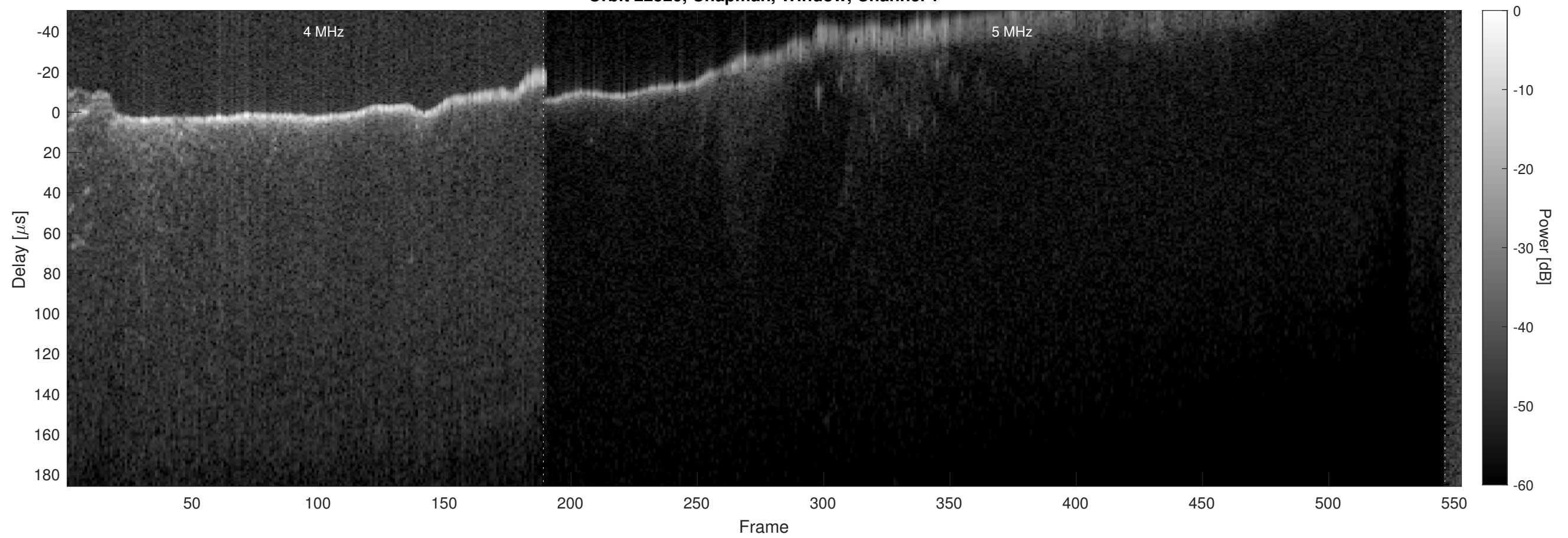
Orbit 22520, Chapman, Window, Channel 2
