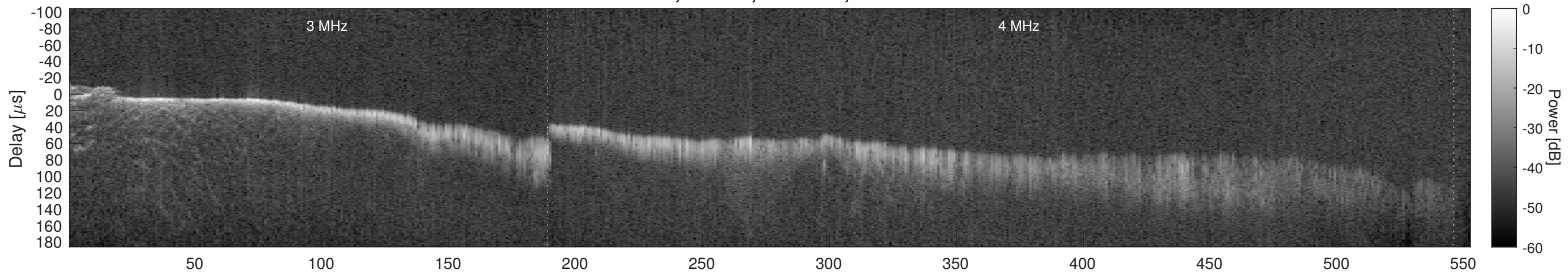
Orbit 22520, Window, Channel 2, Chapman
