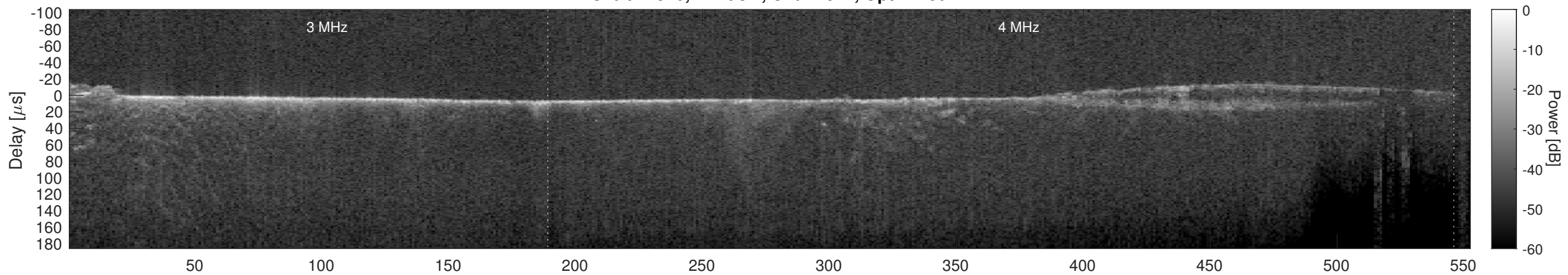
Orbit 22520, Cluttergram
