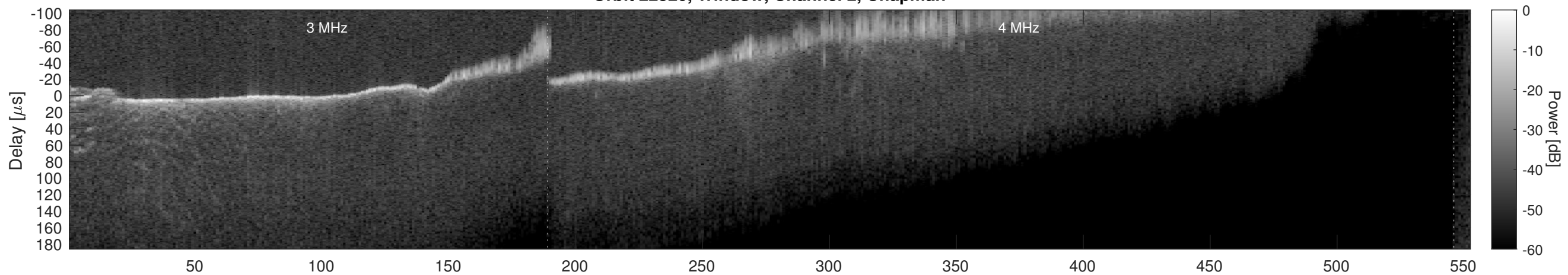
Orbit 22520, Window, Channel 2, Optimized
