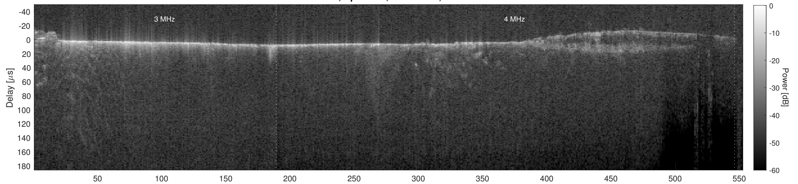
Orbit 22520, Cluttergram
