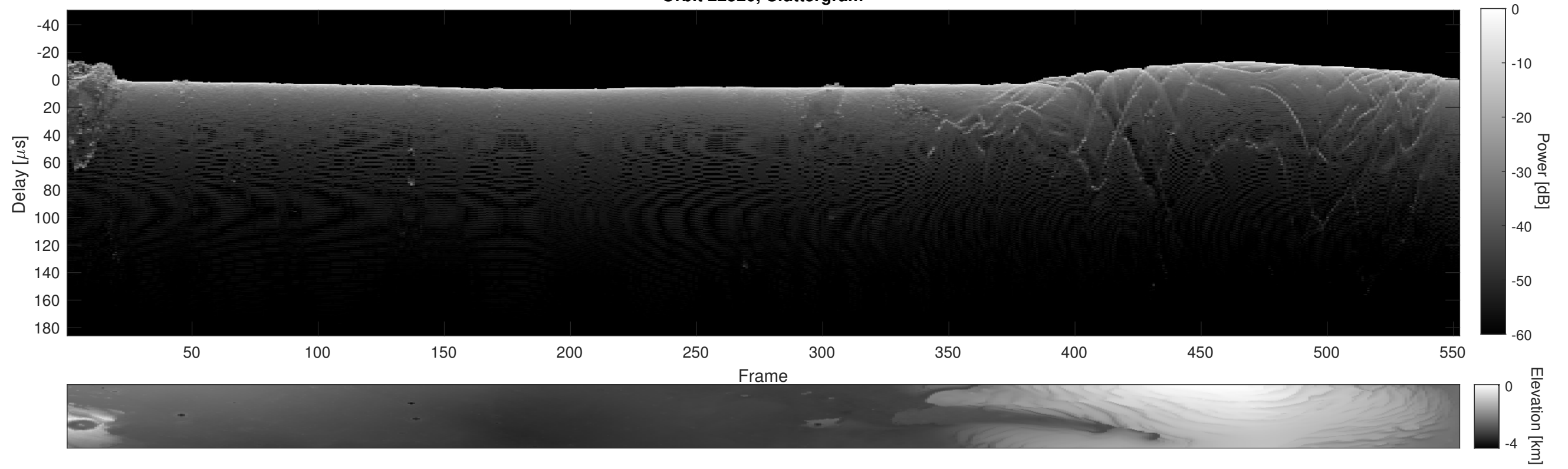
Orbit 22520, Cluttergram
