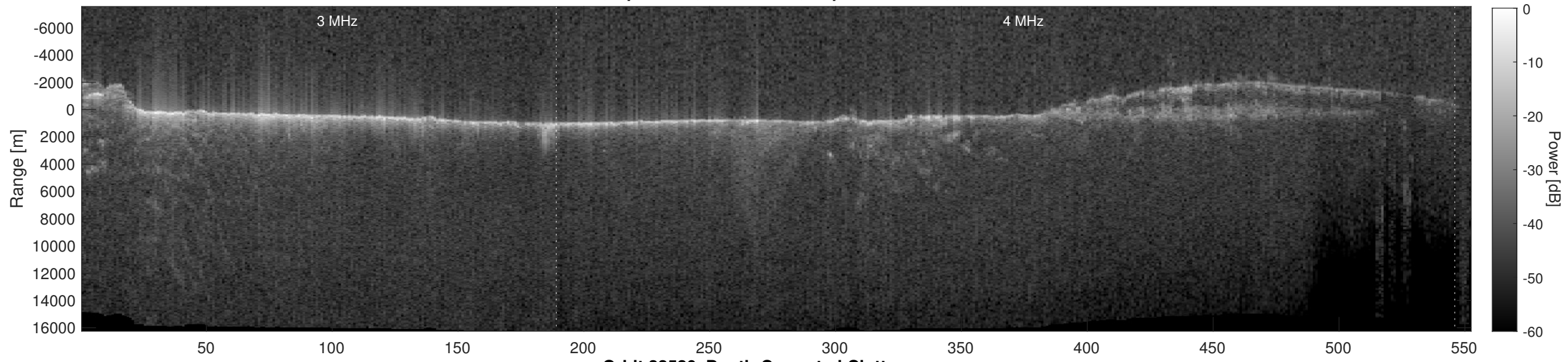
Orbit 22520, Depth-Corrected Cluttergram
