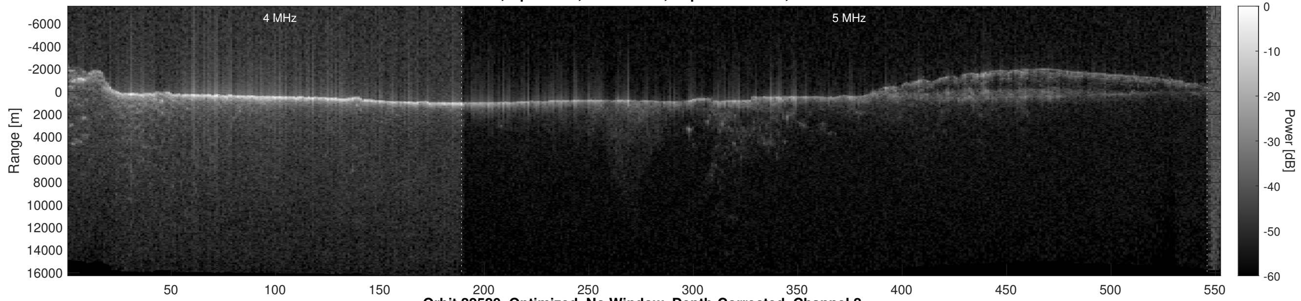
Orbit 22520, Optimized, No Window, Depth-Corrected, Channel 2
