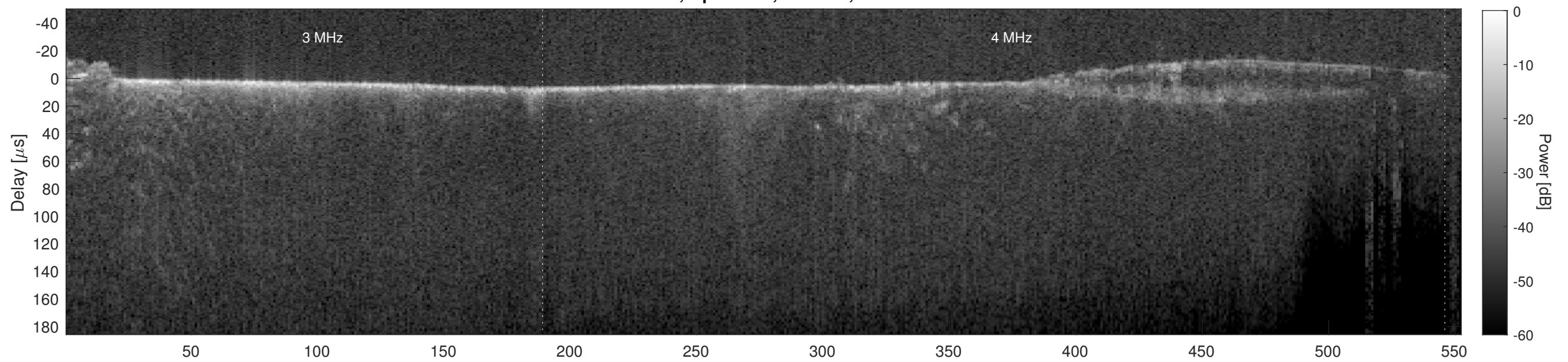
Orbit 22520, Cluttergram
