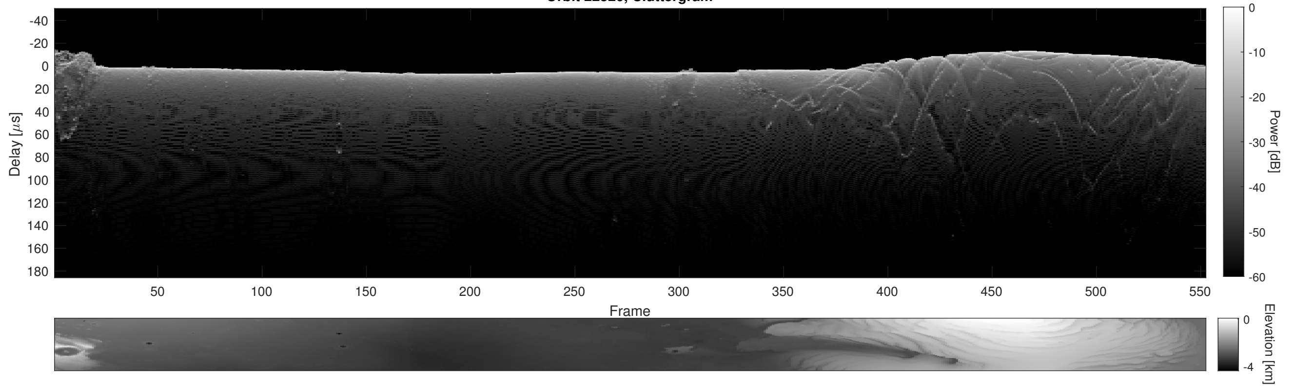
Orbit 22520, Cluttergram
