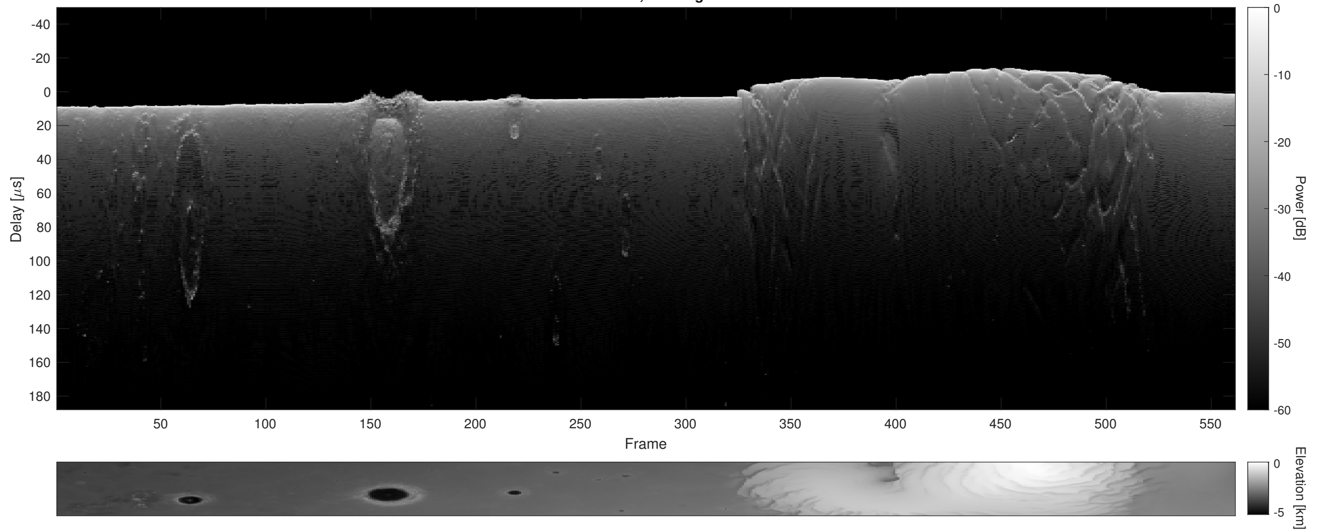
Orbit 22523, Cluttergram
