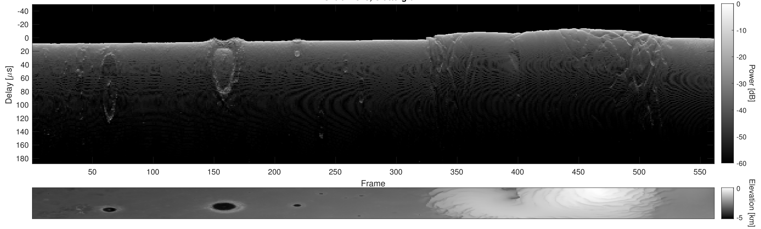
Orbit 22523, Cluttergram
