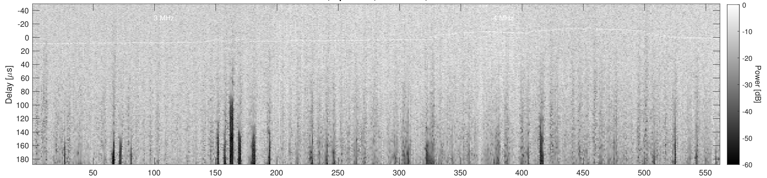
Orbit 22523, Cluttergram
