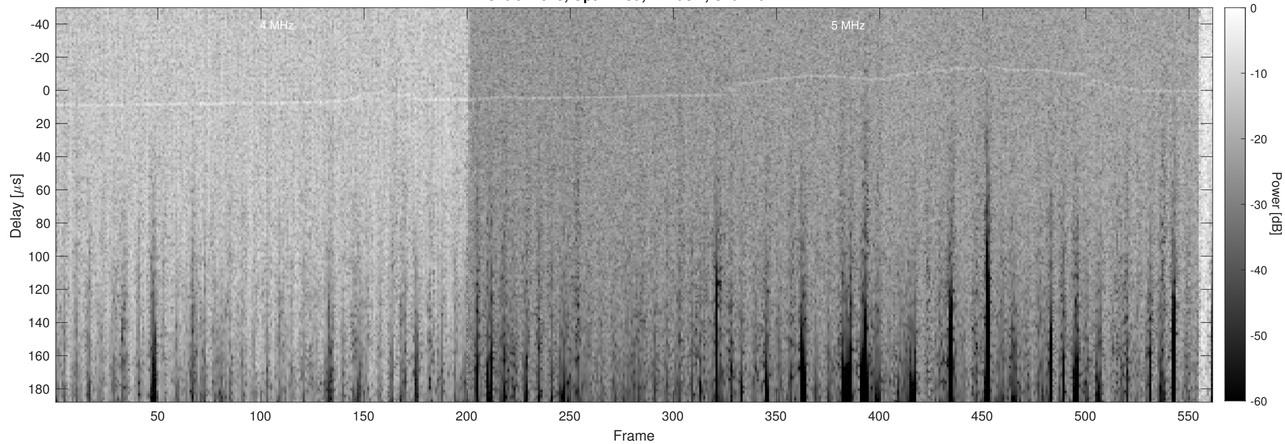
Orbit 22523, Optimized, Window, Channel 2
