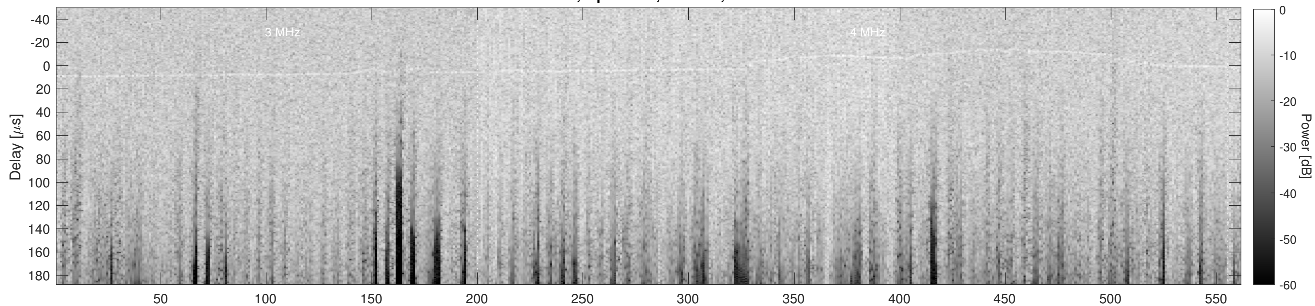
Orbit 22523, Cluttergram
