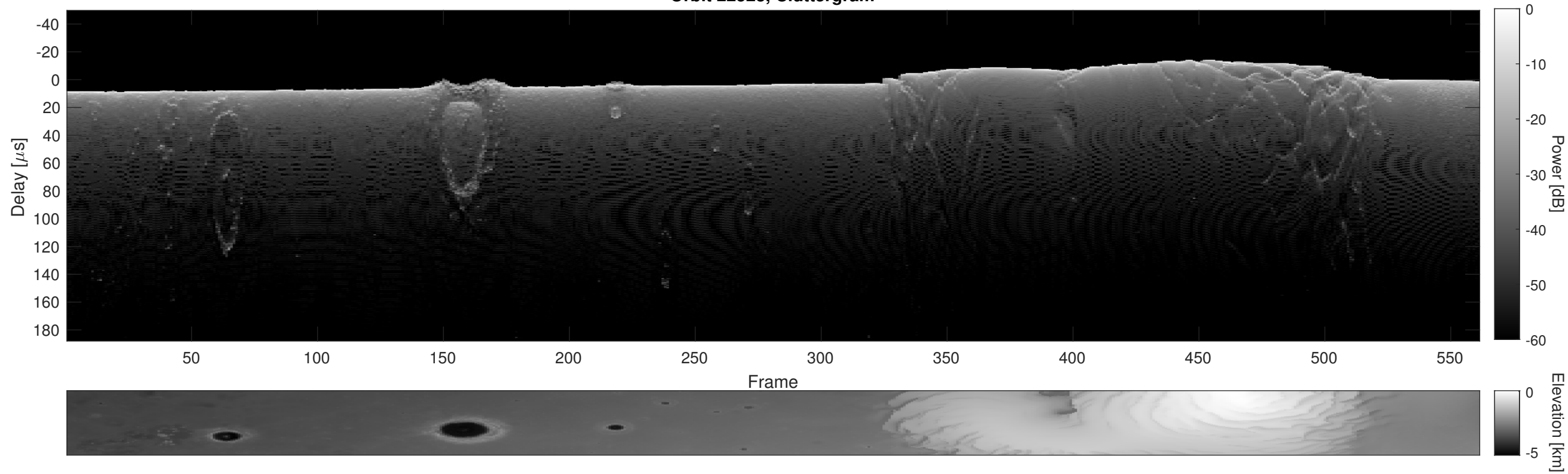
Orbit 22523, Cluttergram
