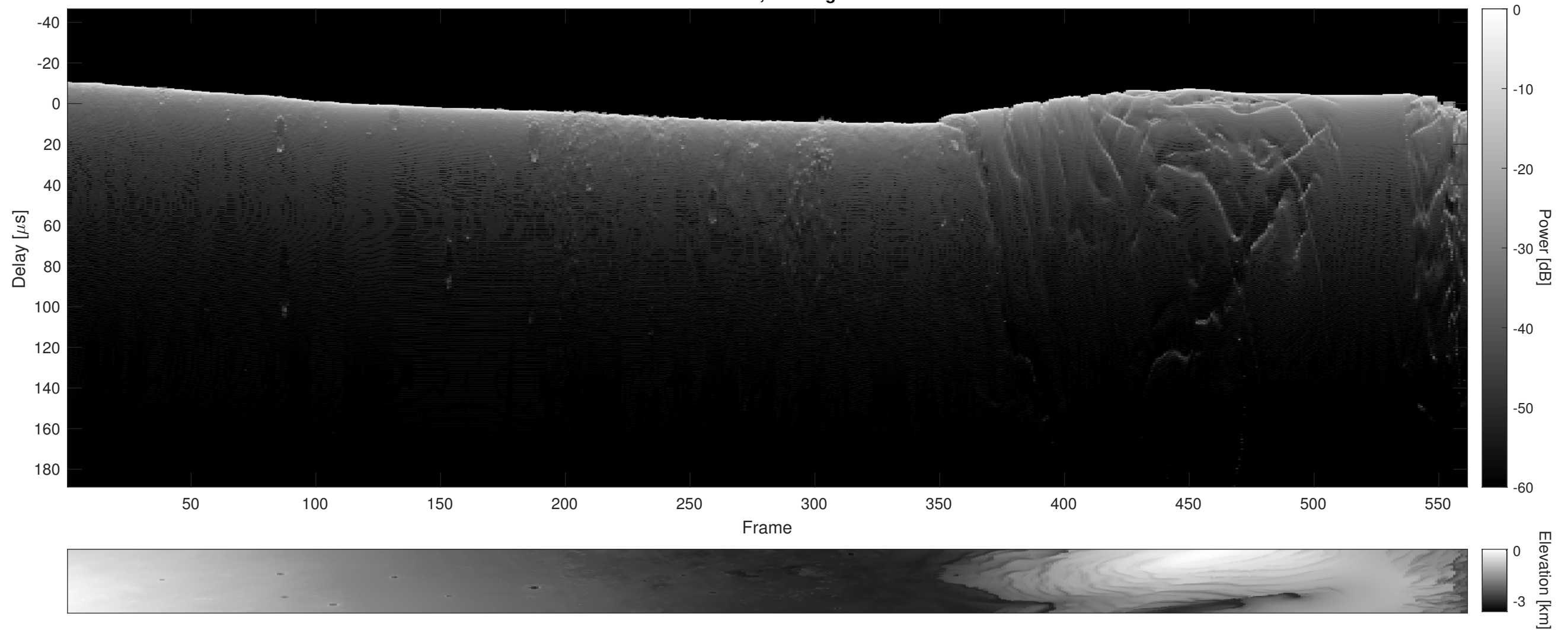
Orbit 22524, Cluttergram
