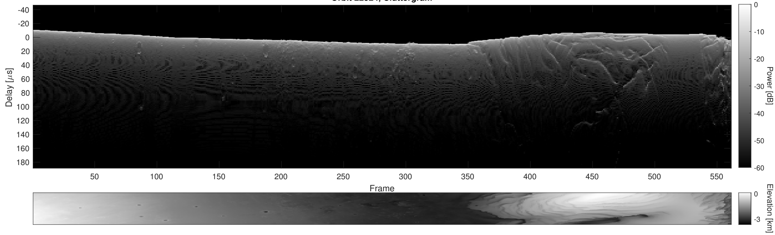
Orbit 22524, Cluttergram
