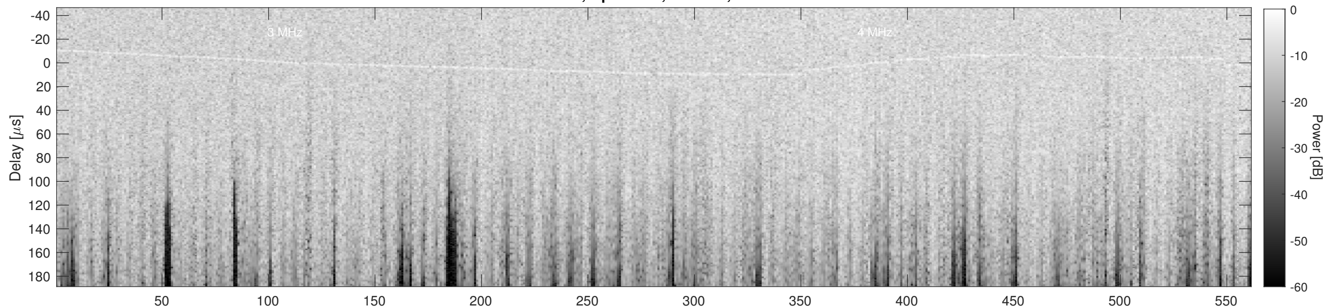
Orbit 22524, Cluttergram
