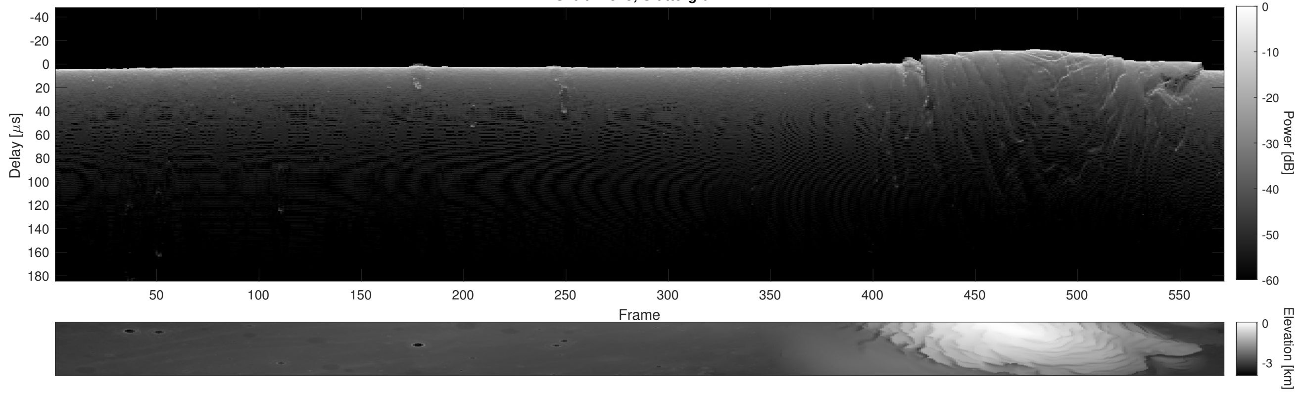
Orbit 22525, Cluttergram
