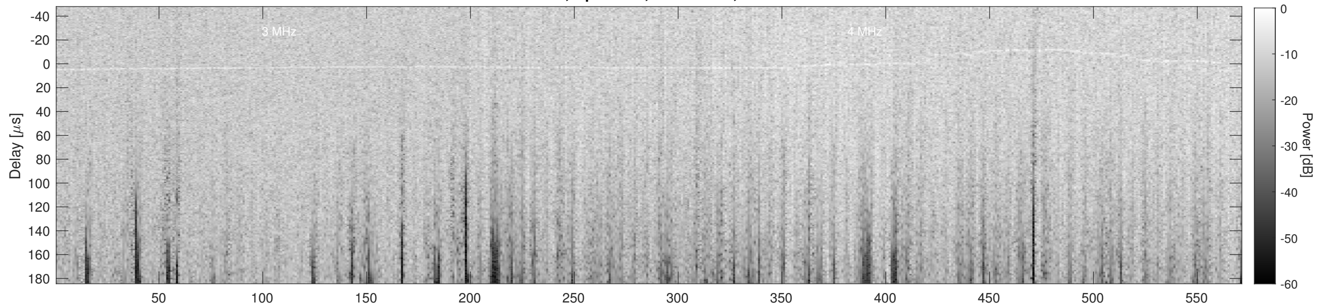
Orbit 22525, Cluttergram
