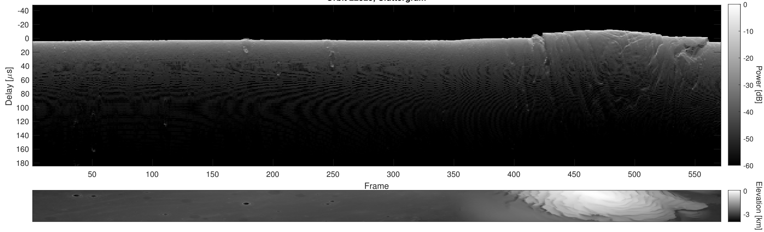
Orbit 22525, Cluttergram
