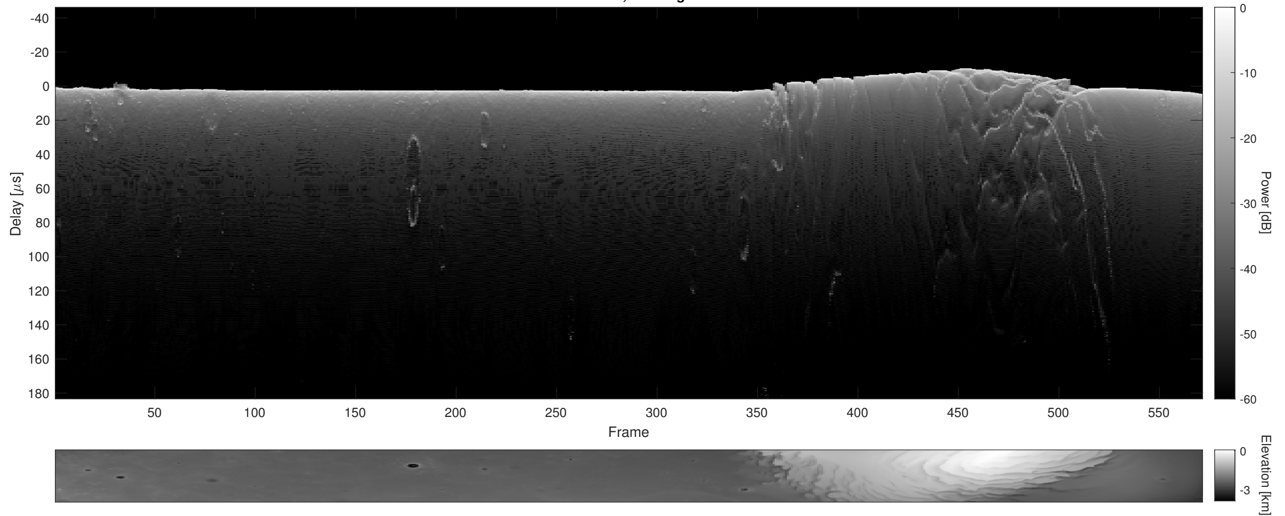
Orbit 22526, Cluttergram
