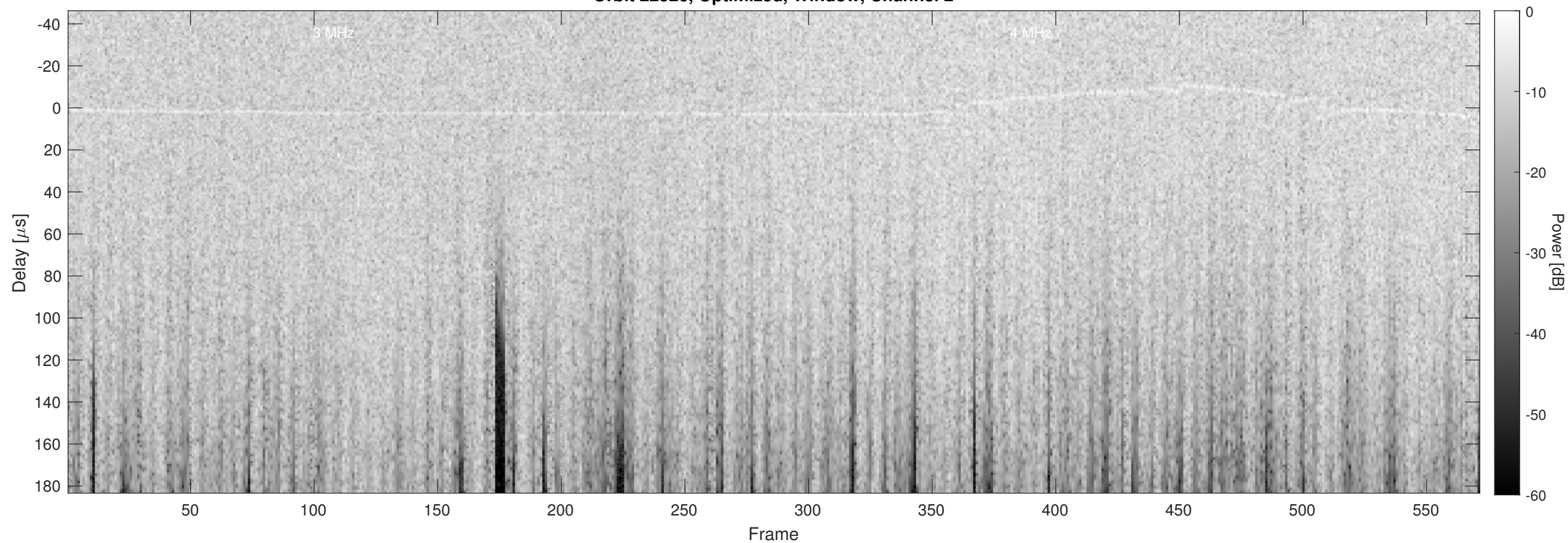
Orbit 22526, Optimized, Window, Channel 2
