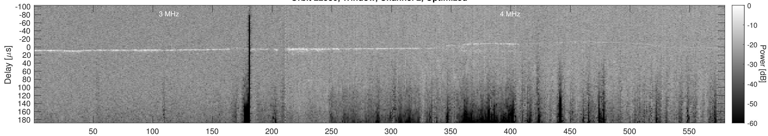
Orbit 22530, Cluttergram
