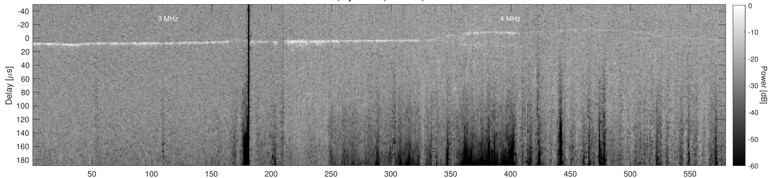
Orbit 22530, Cluttergram
