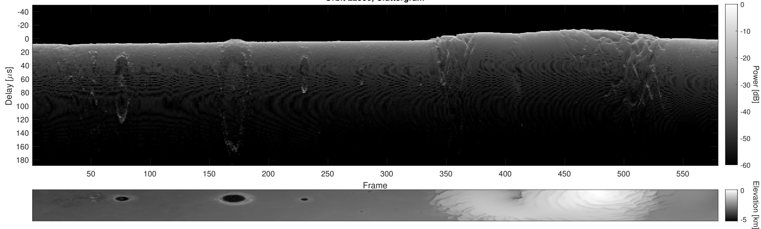
Orbit 22530, Cluttergram
