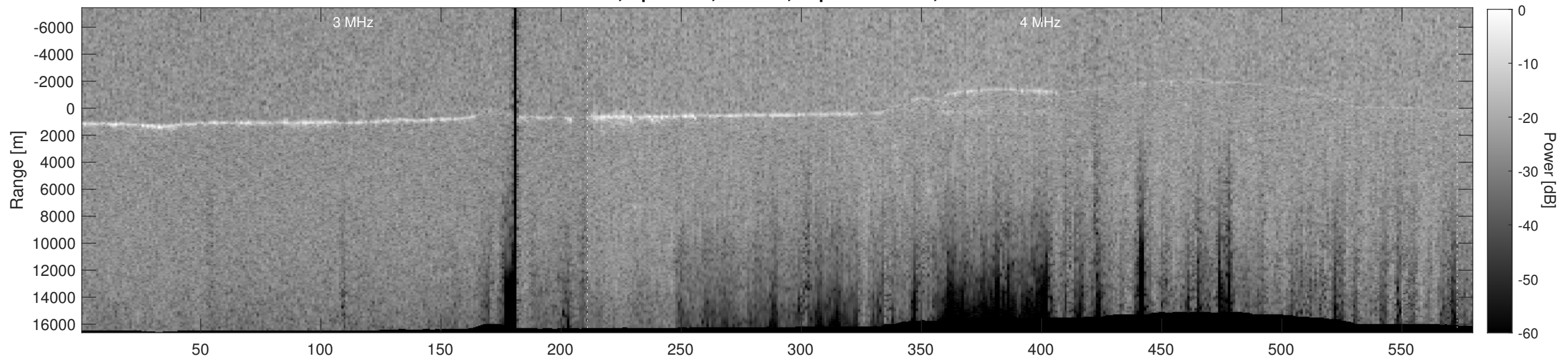
Orbit 22530, Depth-Corrected Cluttergram
