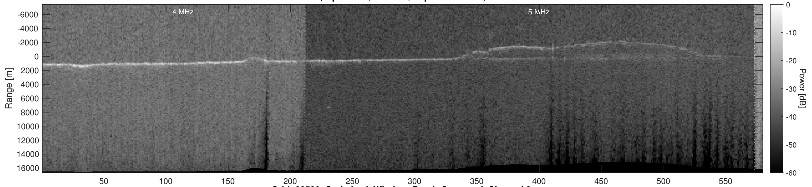
Orbit 22530, Optimized, Window, Depth-Corrected, Channel 2
