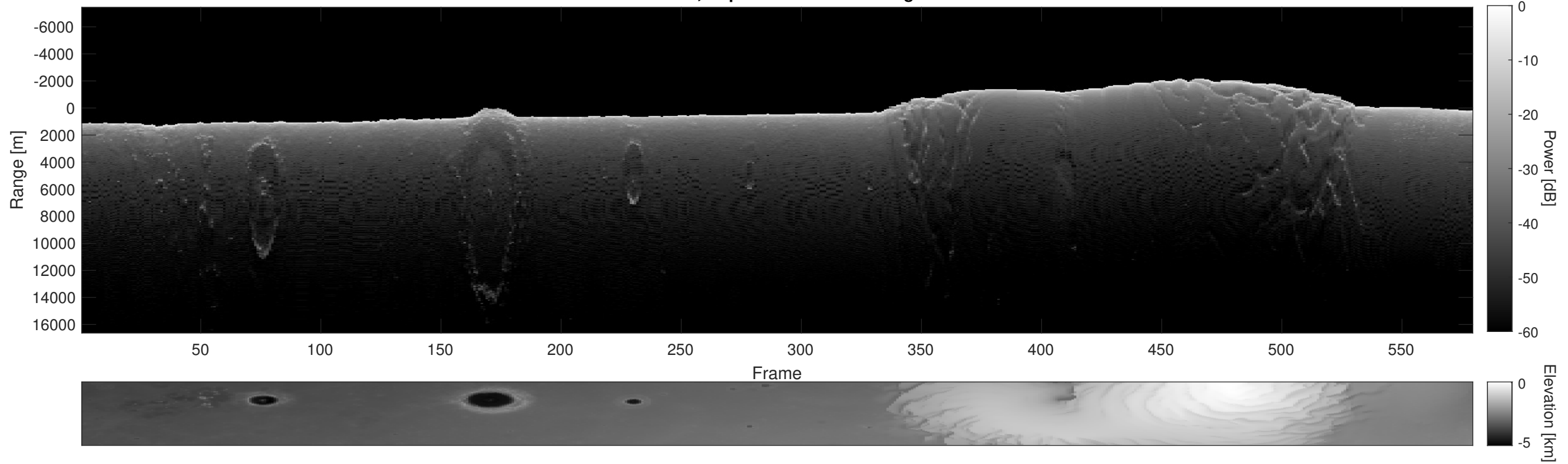
Orbit 22530, Depth-Corrected Cluttergram
