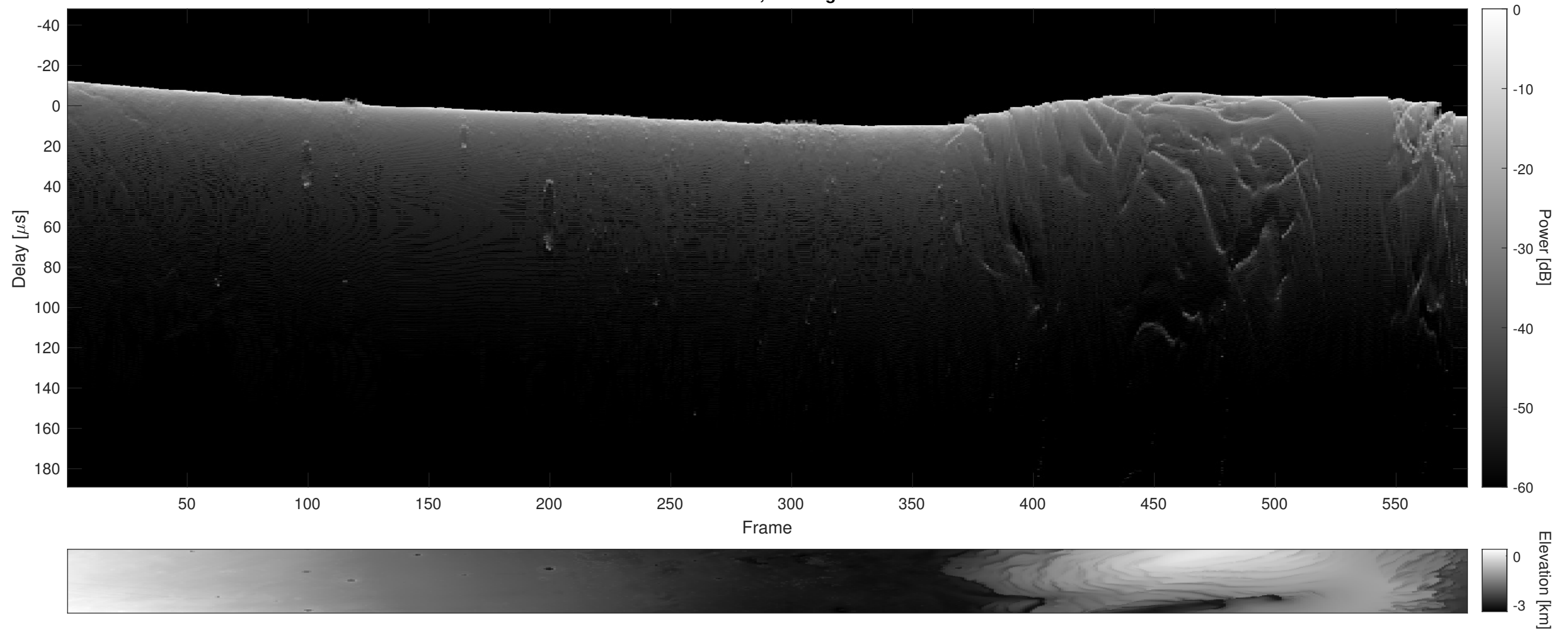
Orbit 22531, Cluttergram
