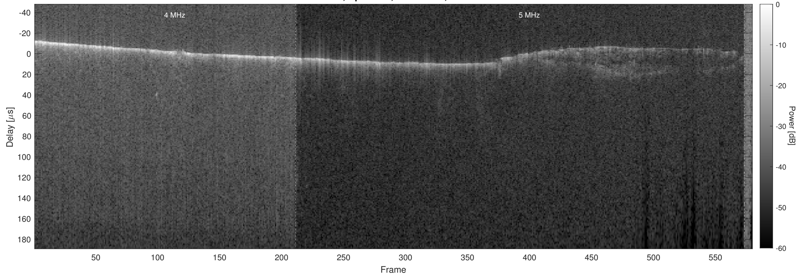
Orbit 22531, Optimized, No Window, Channel 2
