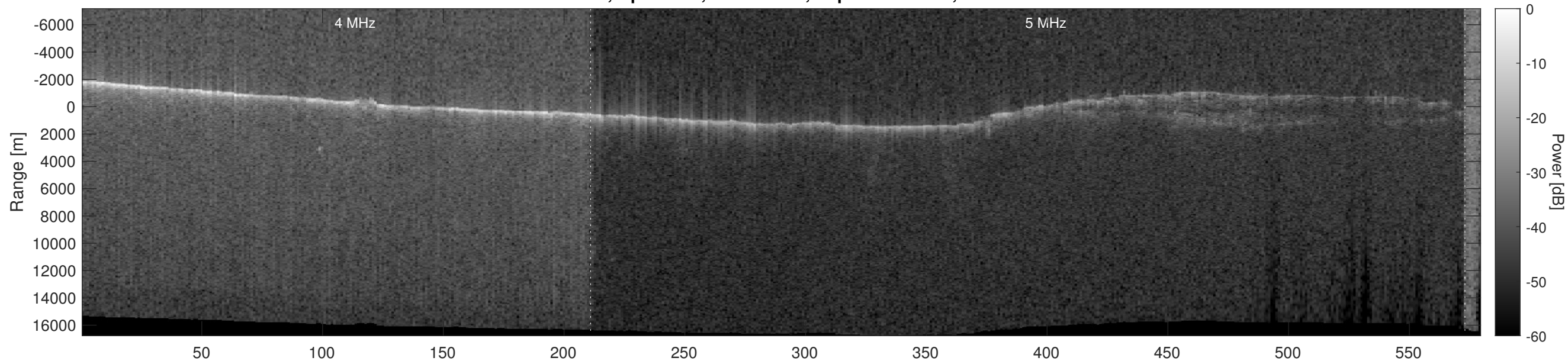
Orbit 22531, Optimized, No Window, Depth-Corrected, Channel 2
