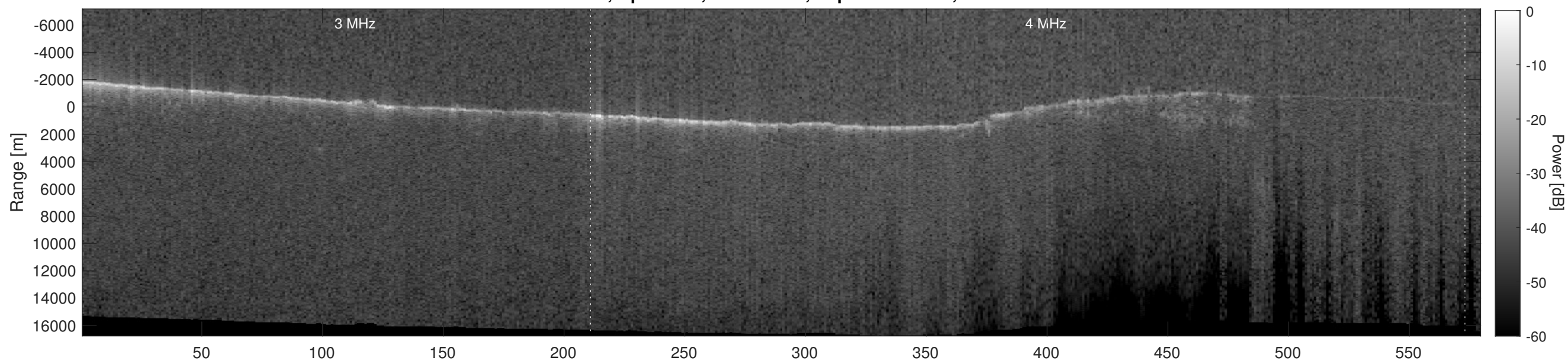
Orbit 22531, Depth-Corrected Cluttergram
