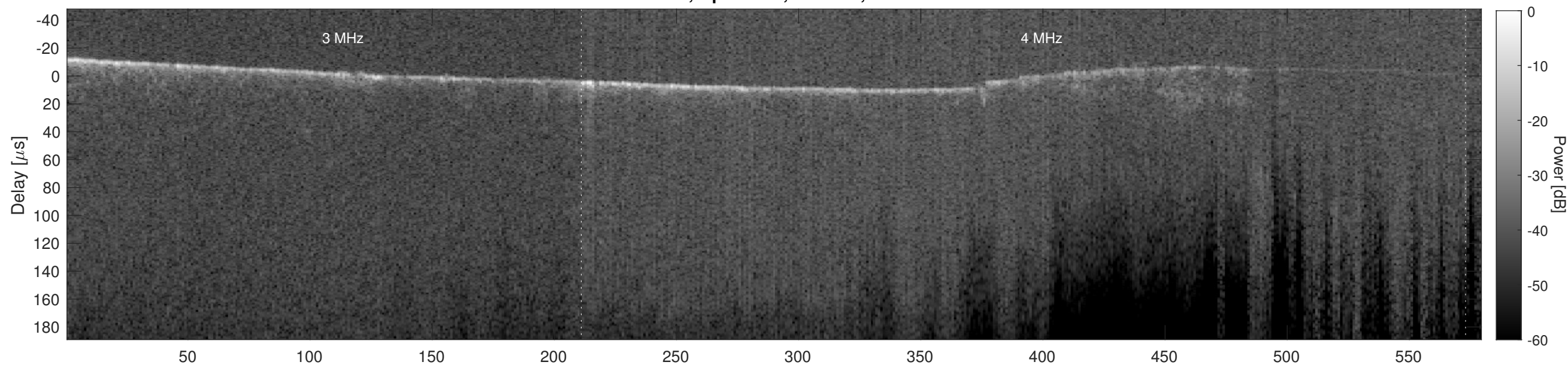
Orbit 22531, Cluttergram
