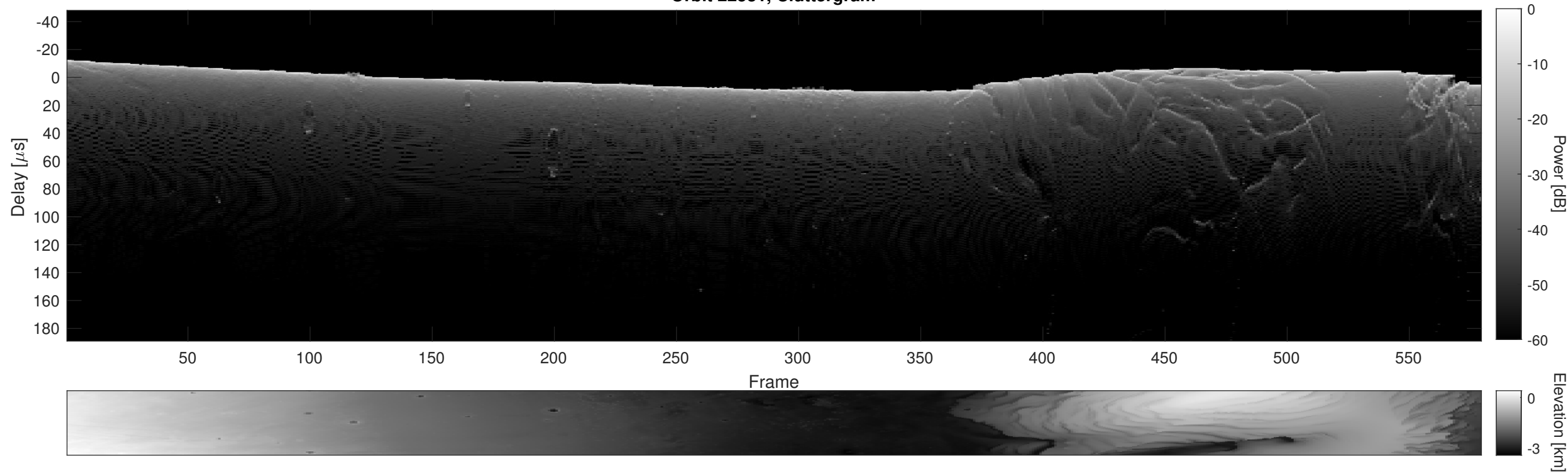
Orbit 22531, Cluttergram
