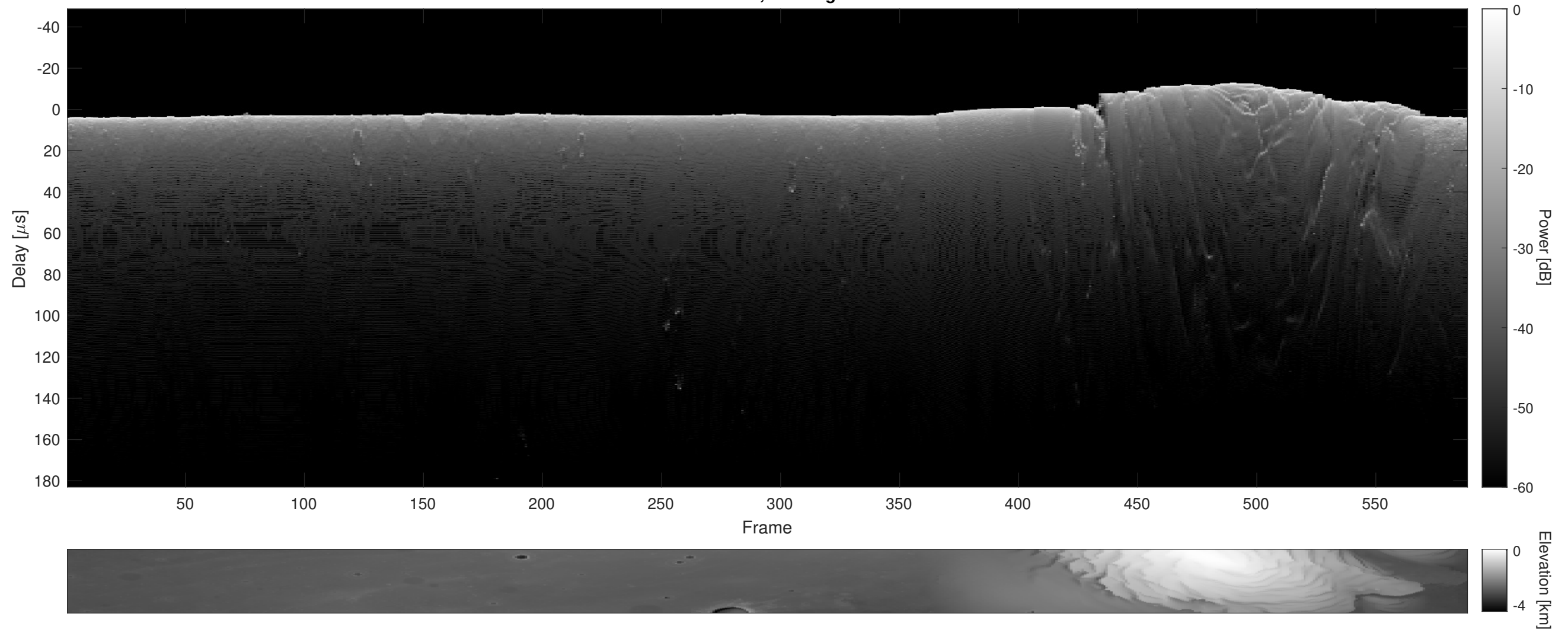
Orbit 22532, Cluttergram
