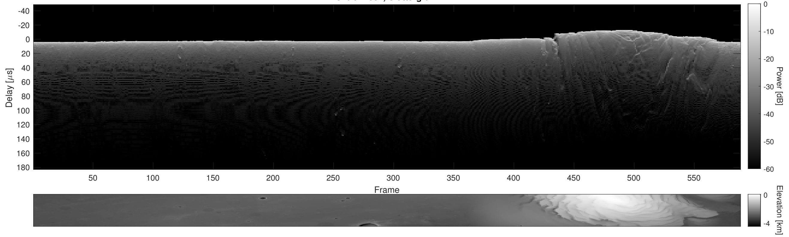
Orbit 22532, Cluttergram
