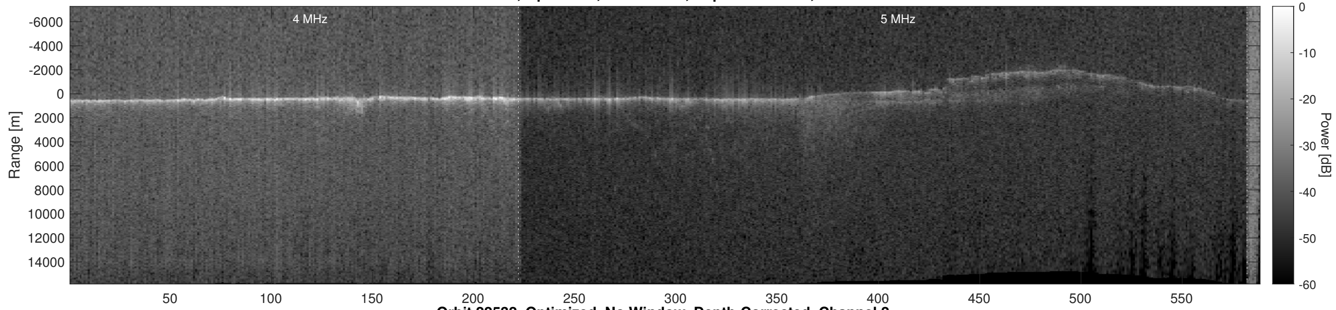
Orbit 22532, Optimized, No Window, Depth-Corrected, Channel 2
