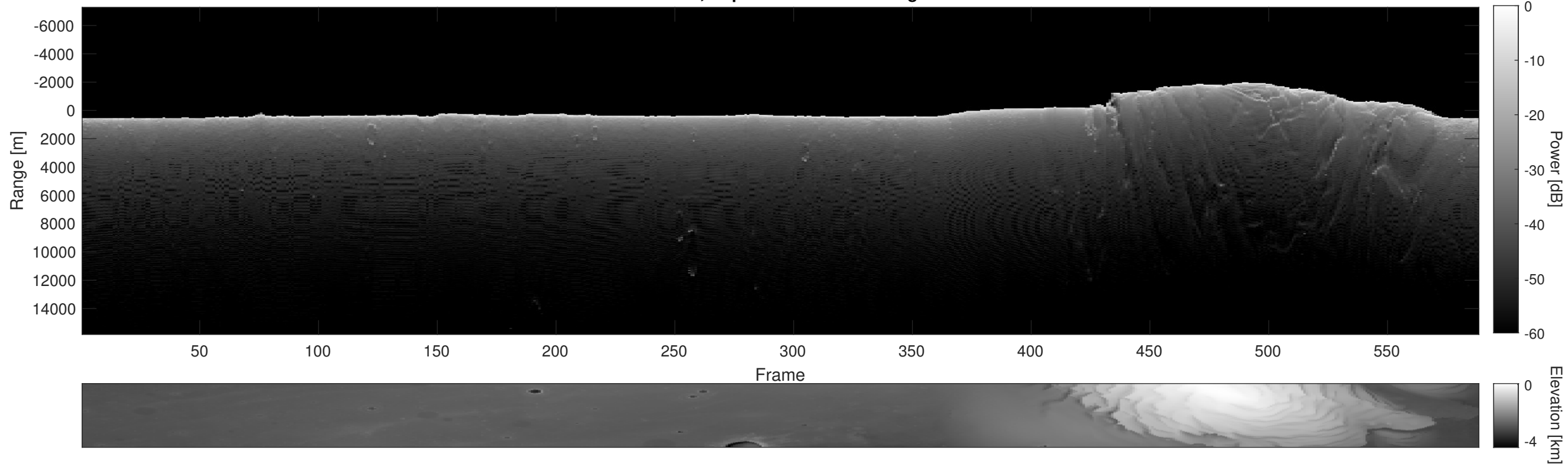
Orbit 22532, Depth-Corrected Cluttergram
