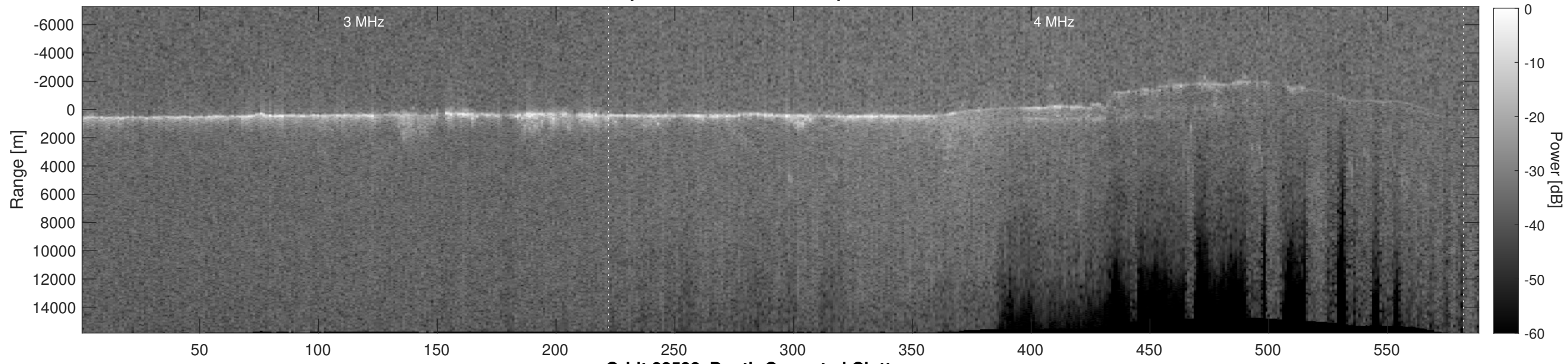
Orbit 22532, Depth-Corrected Cluttergram
