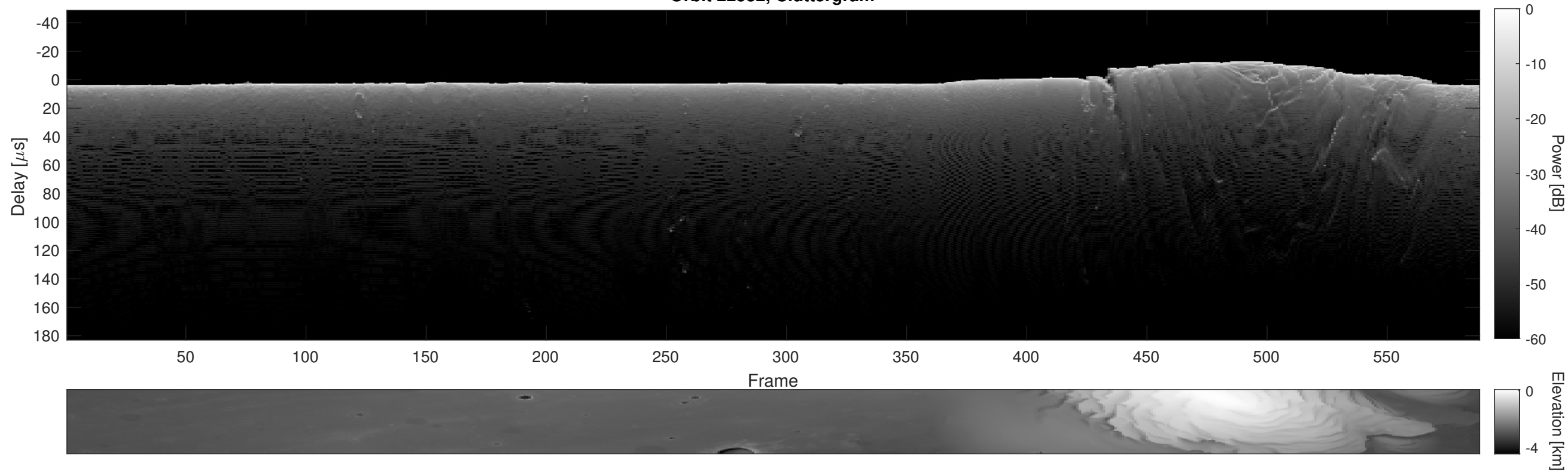
Orbit 22532, Cluttergram
