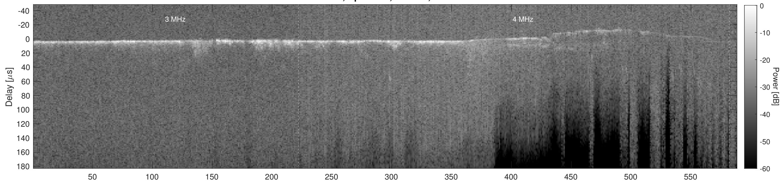
Orbit 22532, Cluttergram
