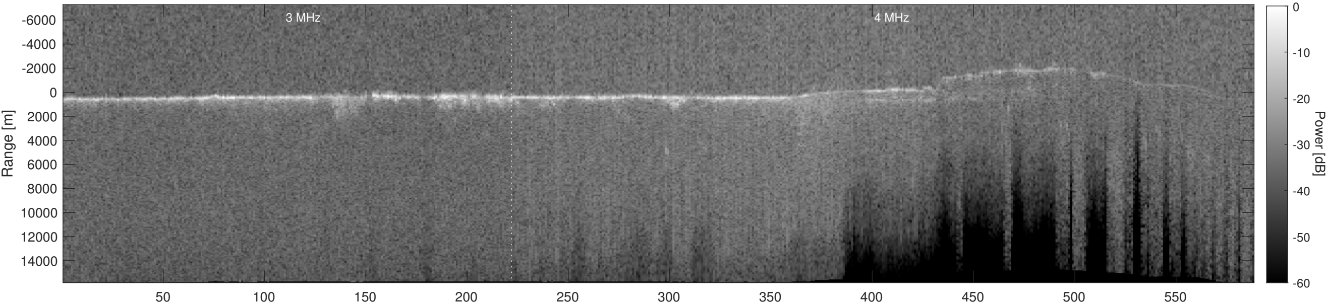
Orbit 22532, Depth-Corrected Cluttergram
