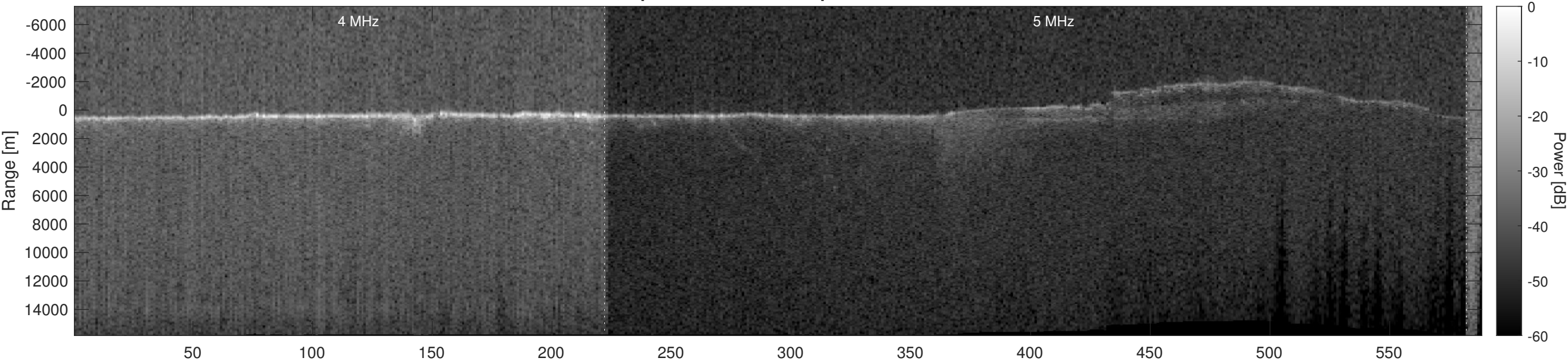
Orbit 22532, Optimized, Window, Depth-Corrected, Channel 2
