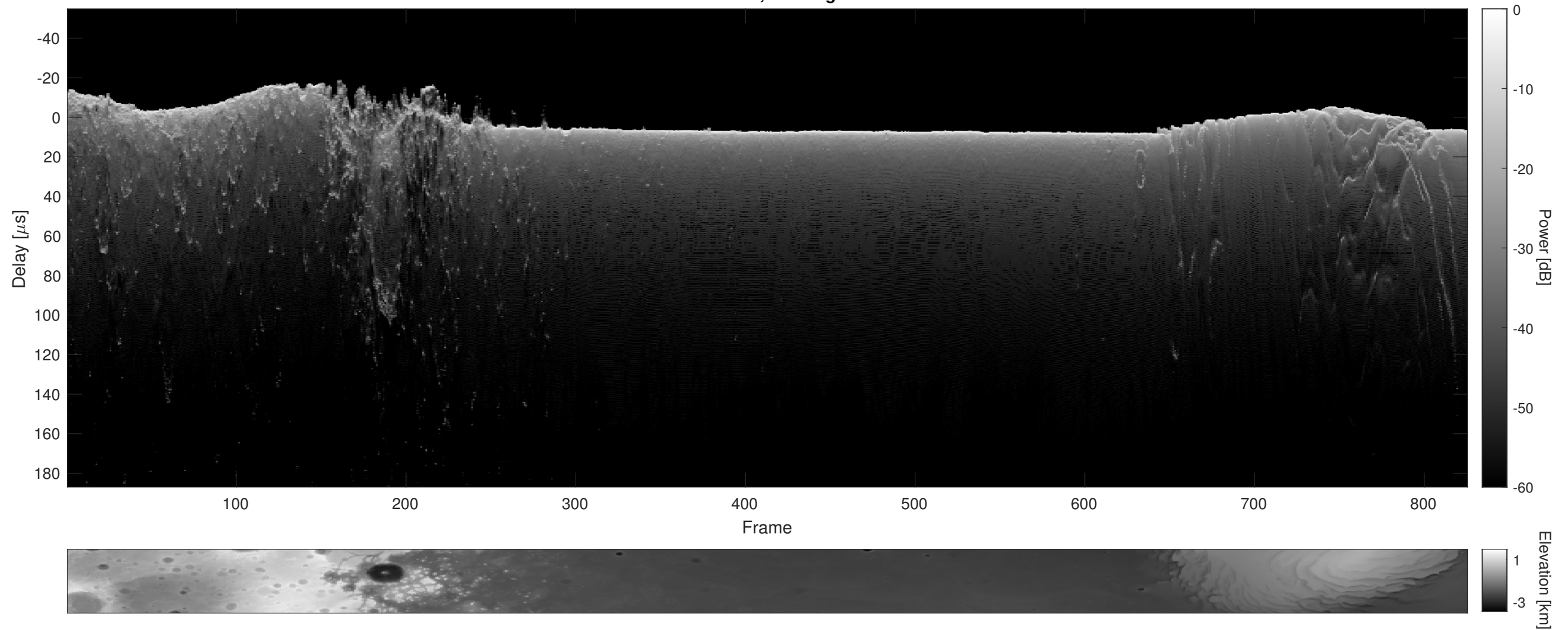
Orbit 22533, Cluttergram
