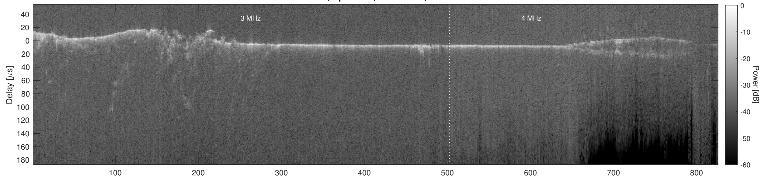
Orbit 22533, Cluttergram
