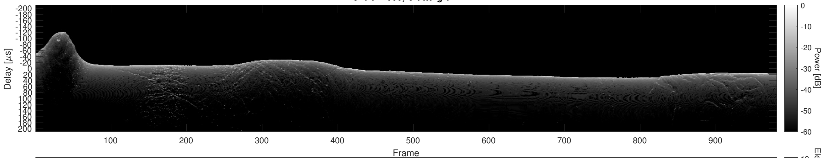
Orbit 22538, Cluttergram
