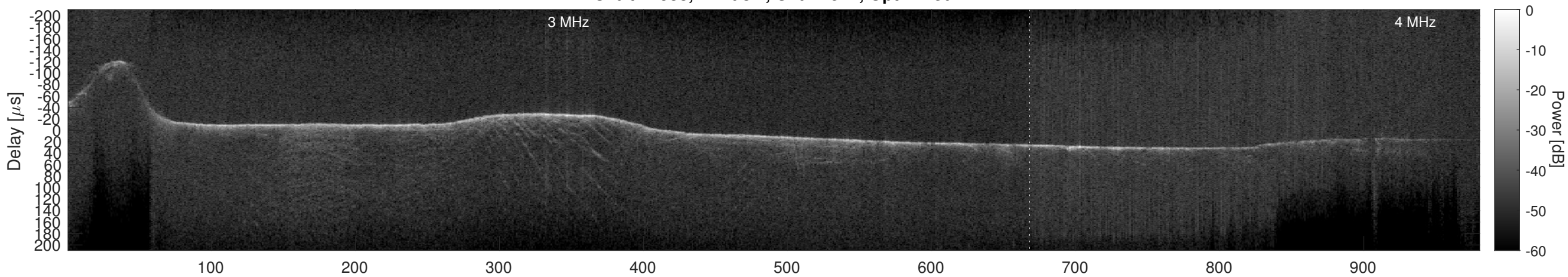
Orbit 22538, Cluttergram
