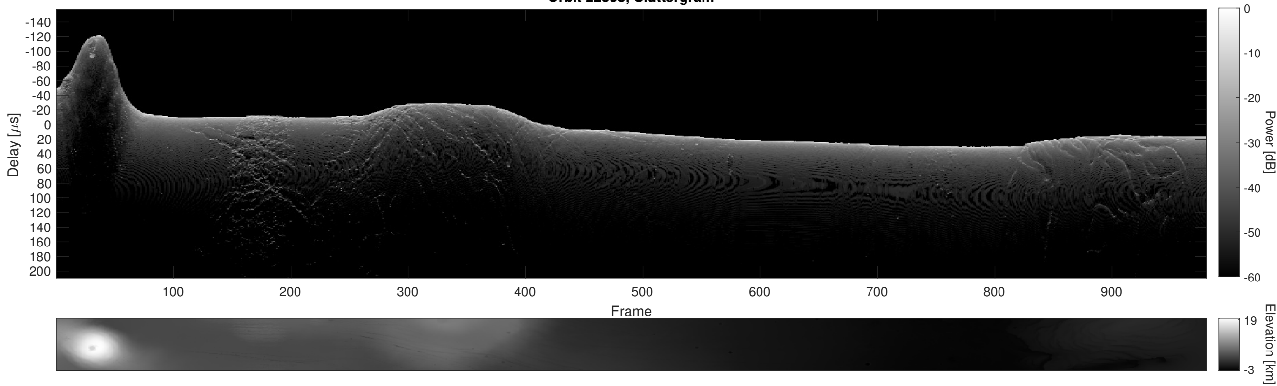
Orbit 22538, Cluttergram
