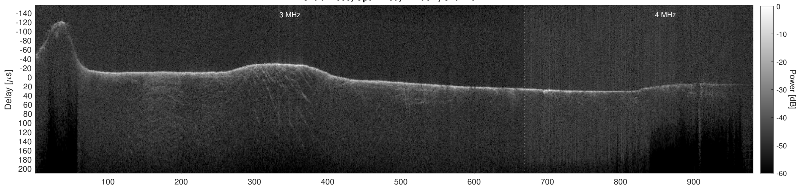
Orbit 22538, Cluttergram
