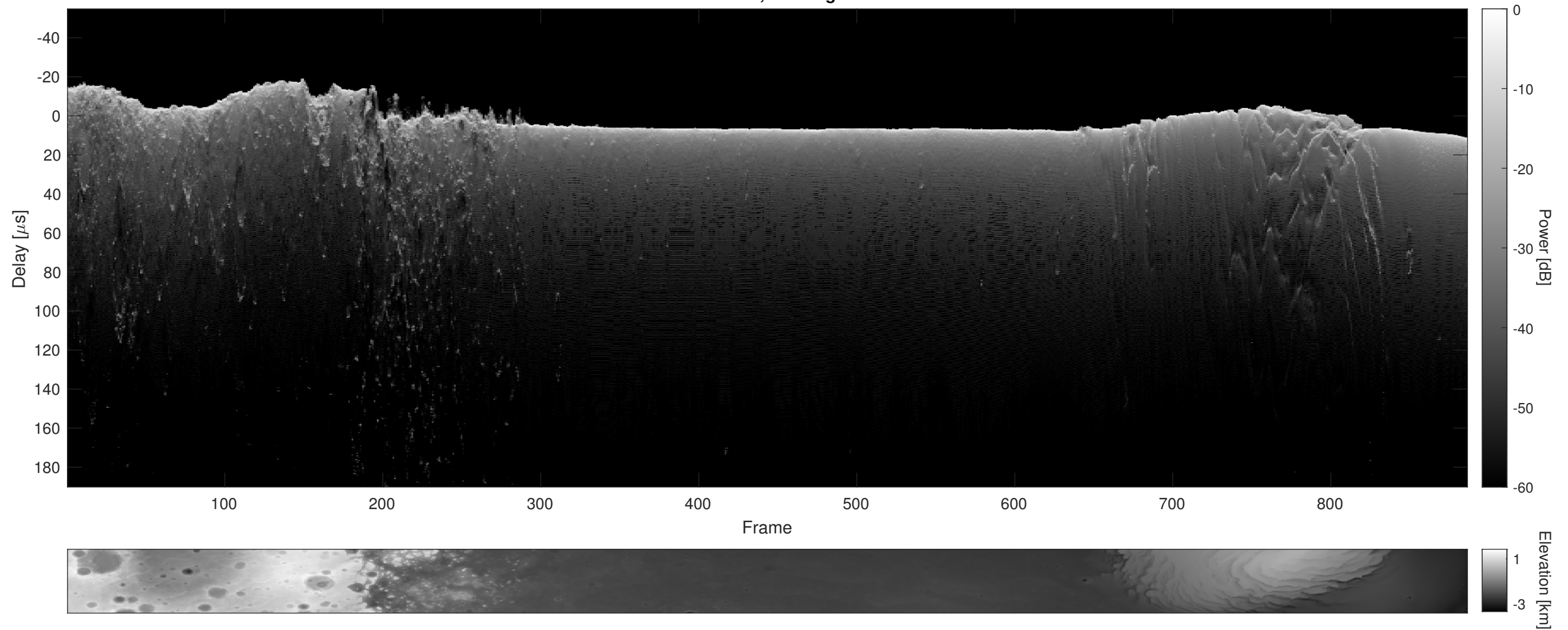
Orbit 22540, Cluttergram
