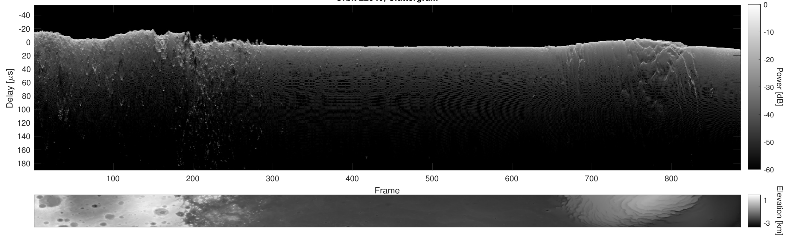
Orbit 22540, Cluttergram
