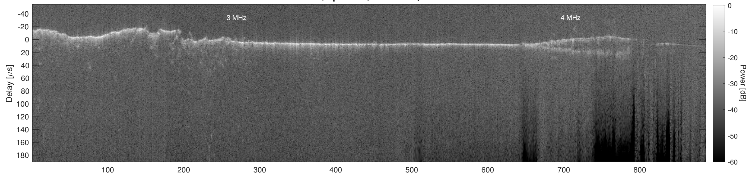
Orbit 22540, Cluttergram
