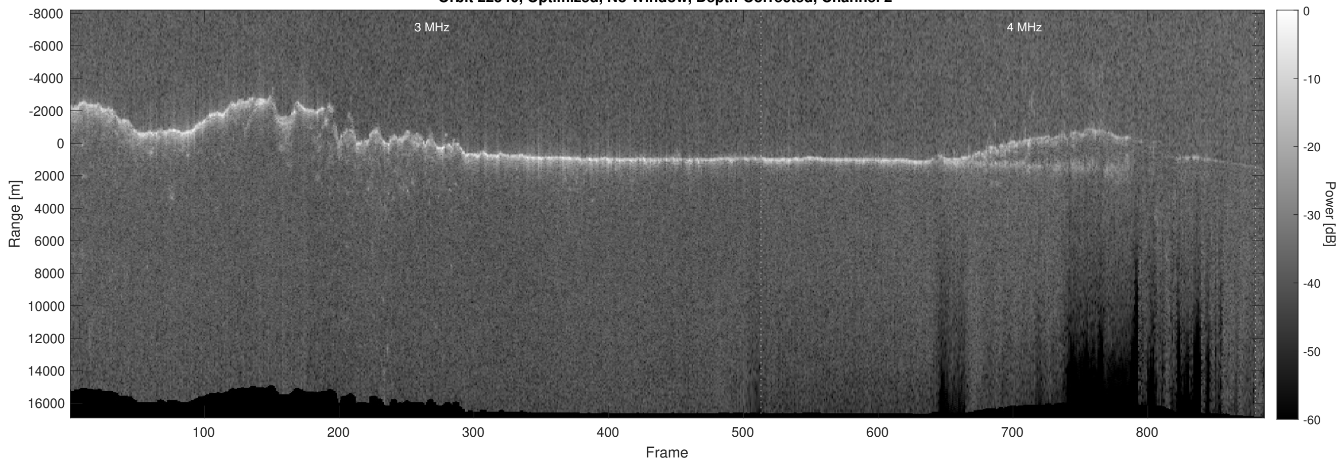
Orbit 22540, Optimized, No Window, Depth-Corrected, Channel 2
