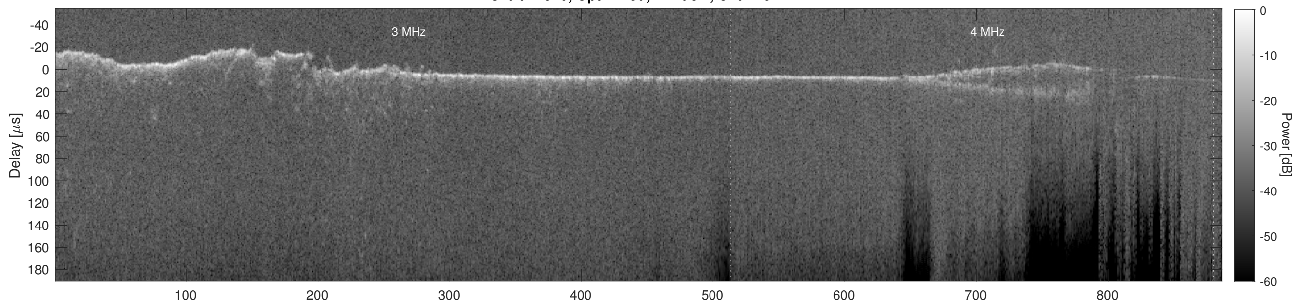
Orbit 22540, Cluttergram
