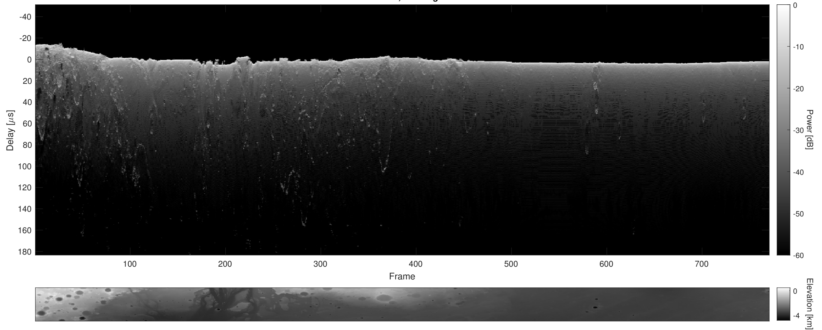
Orbit 22541, Cluttergram
