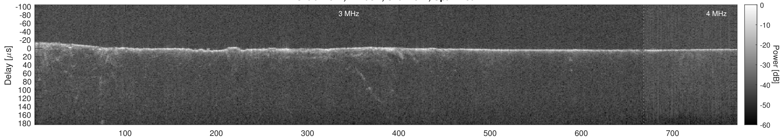
Orbit 22541, Cluttergram
