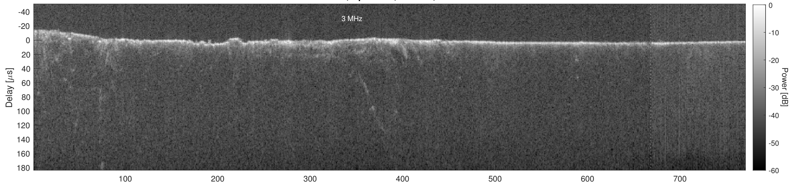
Orbit 22541, Cluttergram
