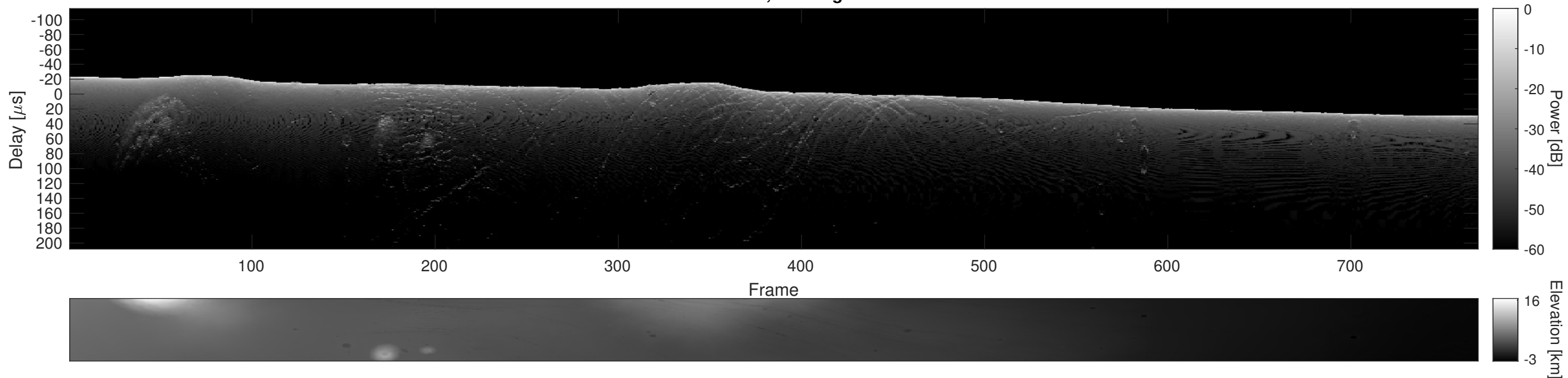
Orbit 22545, Cluttergram
