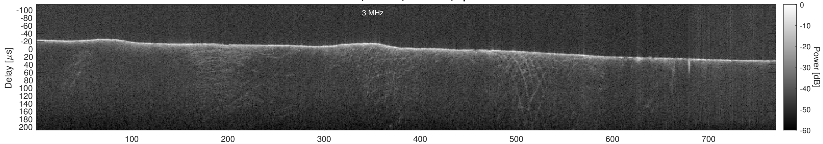
Orbit 22545, Cluttergram
