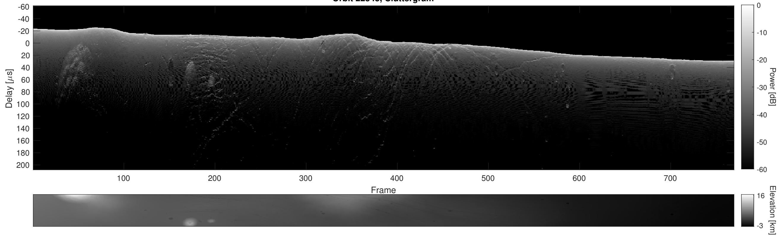
Orbit 22545, Cluttergram
