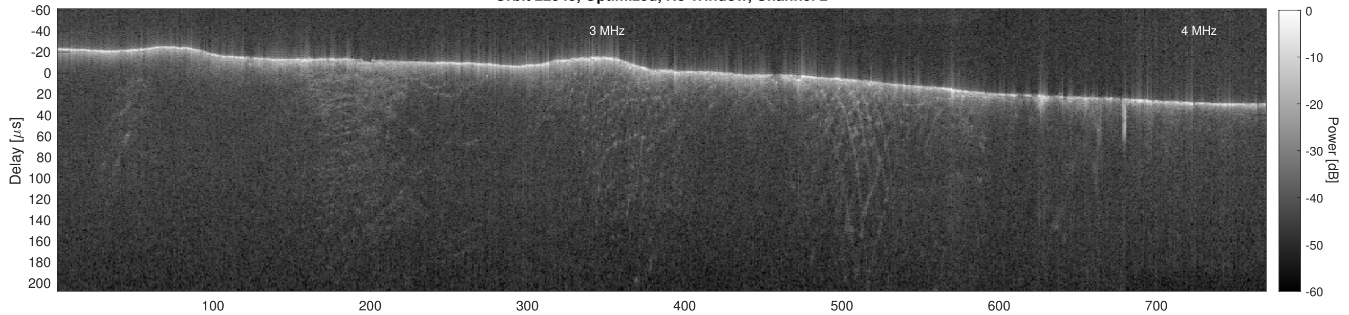
Orbit 22545, Cluttergram
