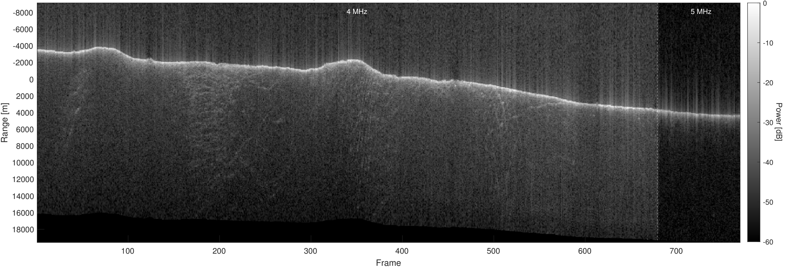
Orbit 22545, Optimized, No Window, Depth-Corrected, Channel 2
