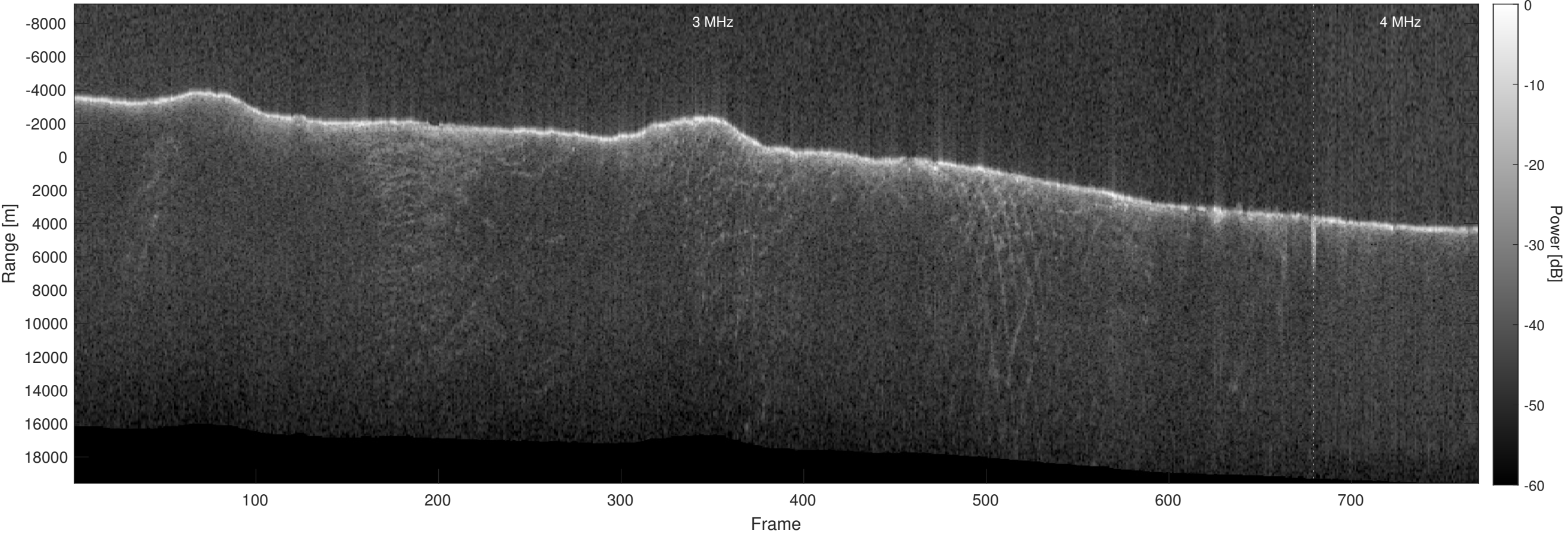
Orbit 22545, Optimized, Window, Depth-Corrected, Channel 2
