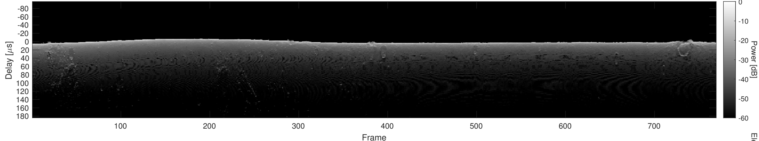
Orbit 22546, Cluttergram
