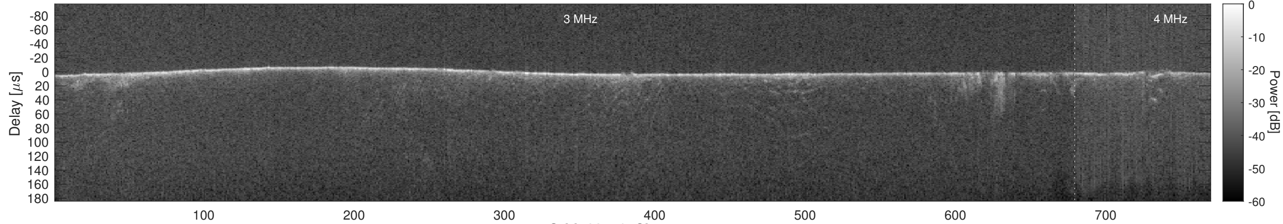
Orbit 22546, Cluttergram
