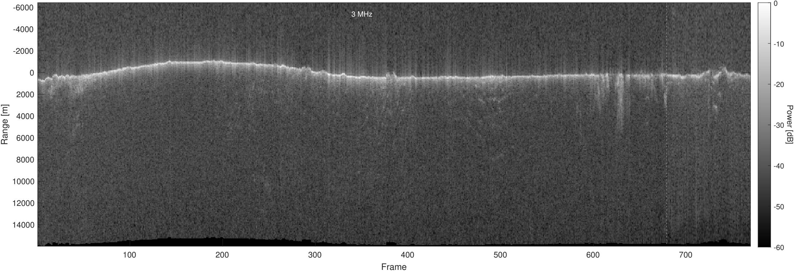
Orbit 22546, Optimized, No Window, Depth-Corrected, Channel 2
