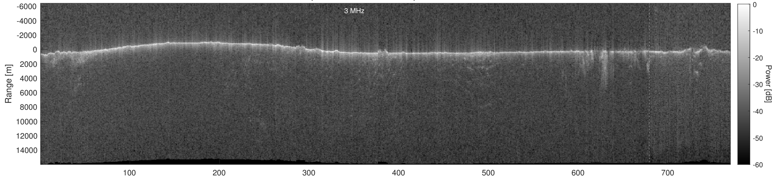
Orbit 22546, Depth-Corrected Cluttergram
