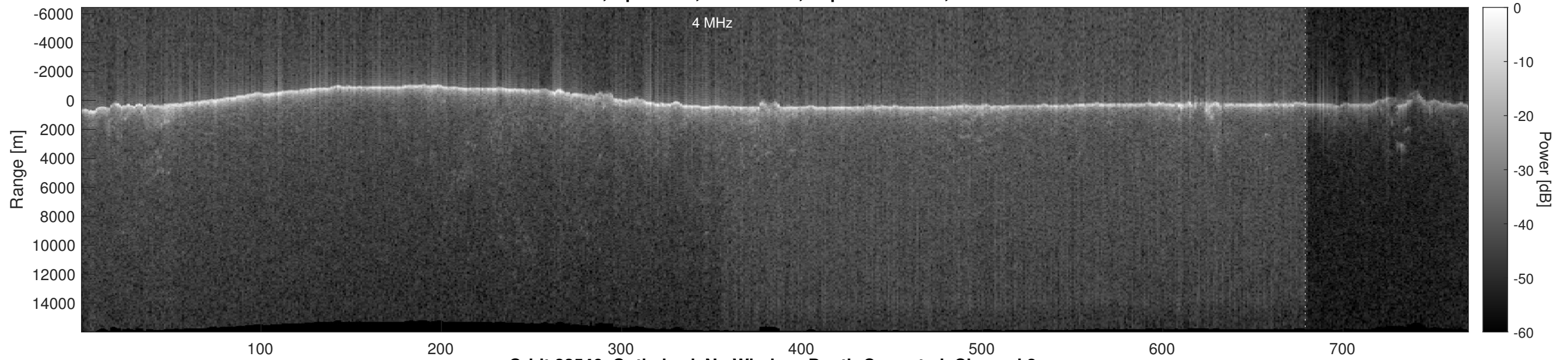
Orbit 22546, Optimized, No Window, Depth-Corrected, Channel 2
