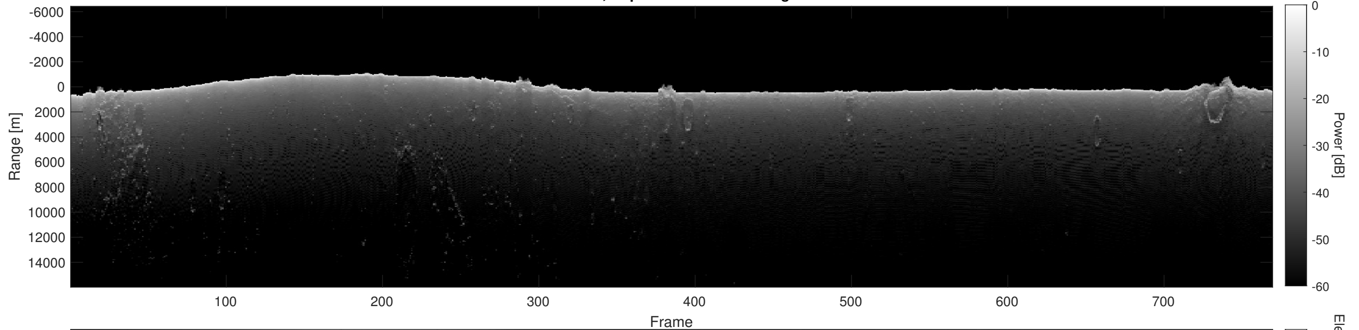
Orbit 22546, Depth-Corrected Cluttergram
